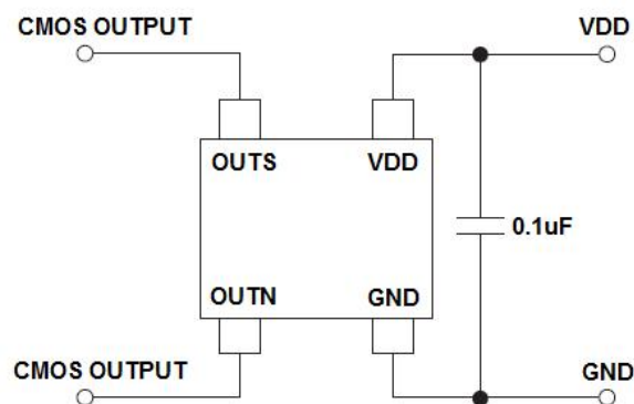
Figure 1, Typical Application Circuit of AS1818
