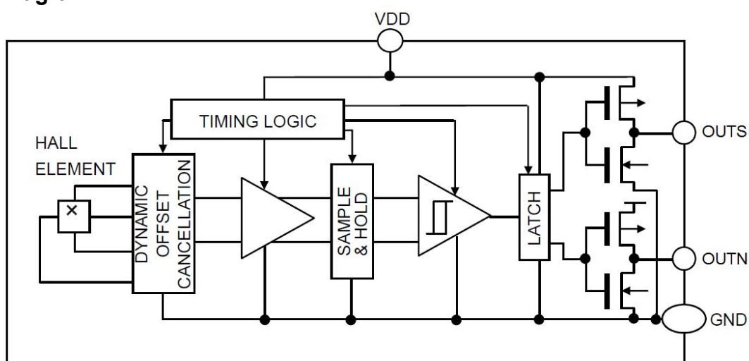
Figure 3, Block Diagram of AS1818
