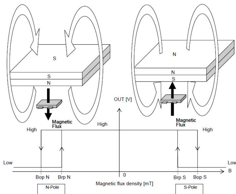
Fig 4, Magnetic Operation Characteristic of AS1818
